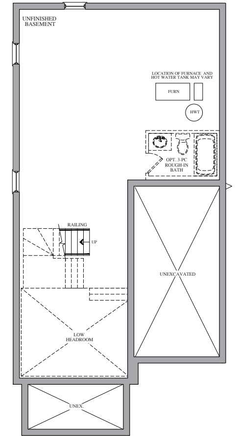
BASEMENT ELEVATION A & B
