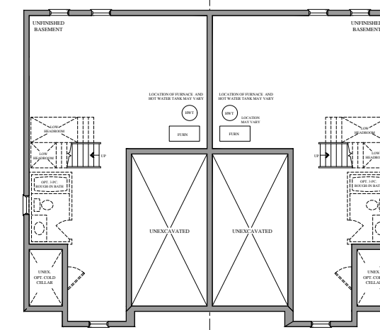
BASEMENT FLOOR PLAN ELEV. 'A', 'B' & 'C'
