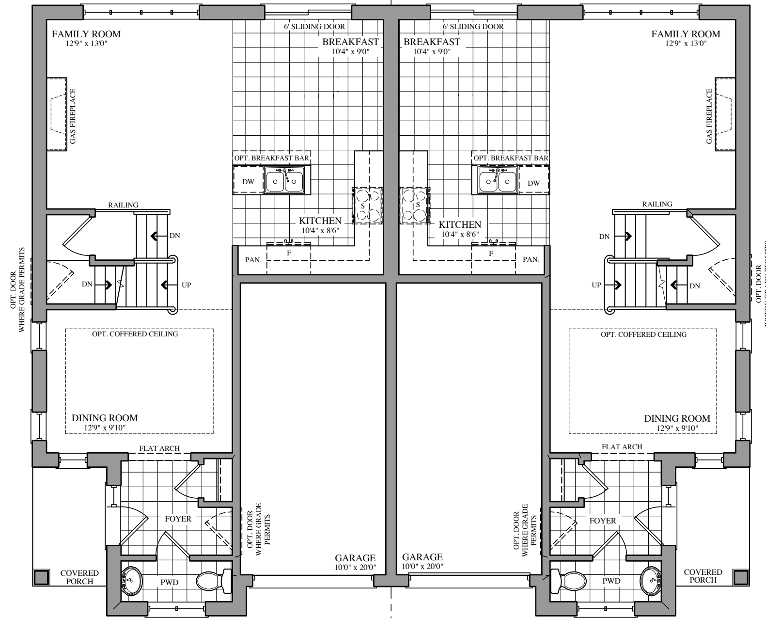
GROUND FLOOR PLAN ELEV. 'A'
