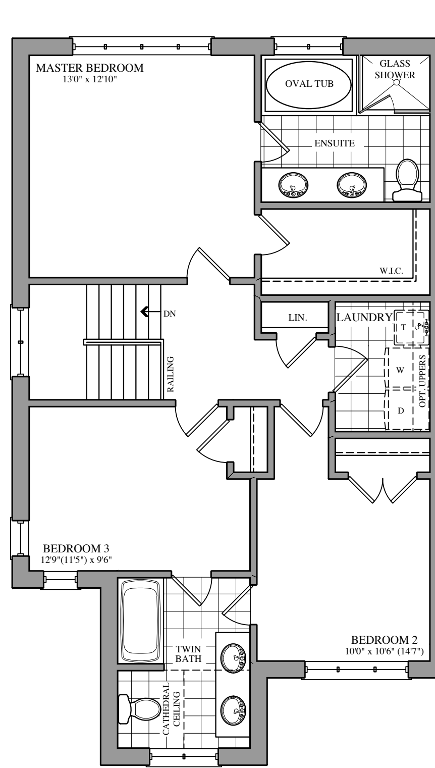
SECOND FLOOR PLAN ELEV. 'A'
