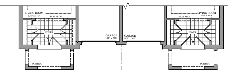
PART. GROUND FLOOR PLAN ELEV. 'C'
