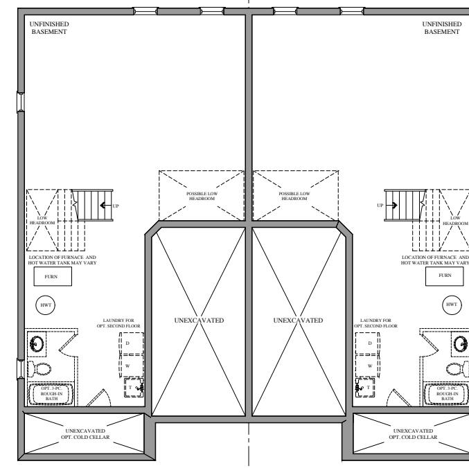
BASEMENT FLOOR PLAN ELEV. 'A'
