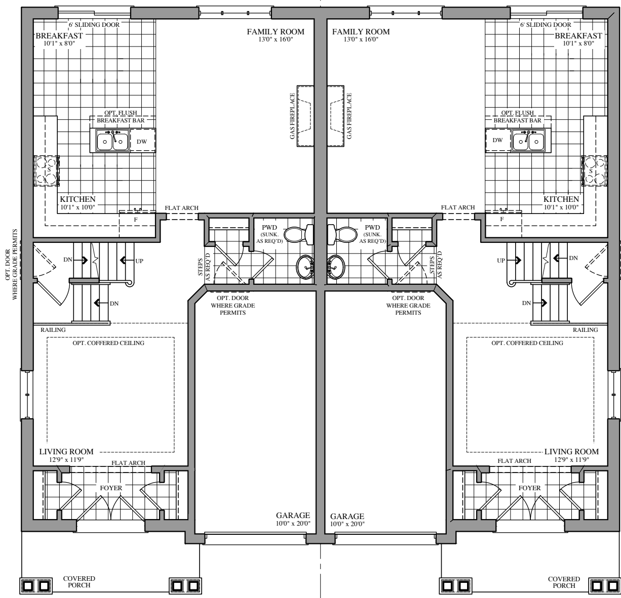
GROUND FLOOR PLAN ELEV. 'A'
