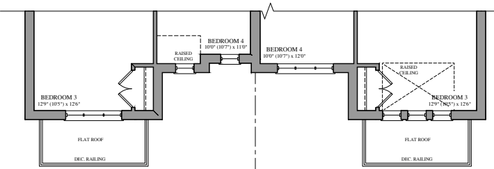
PART. OPT. SECOND FLOOR PLAN ELEV. 'C'
