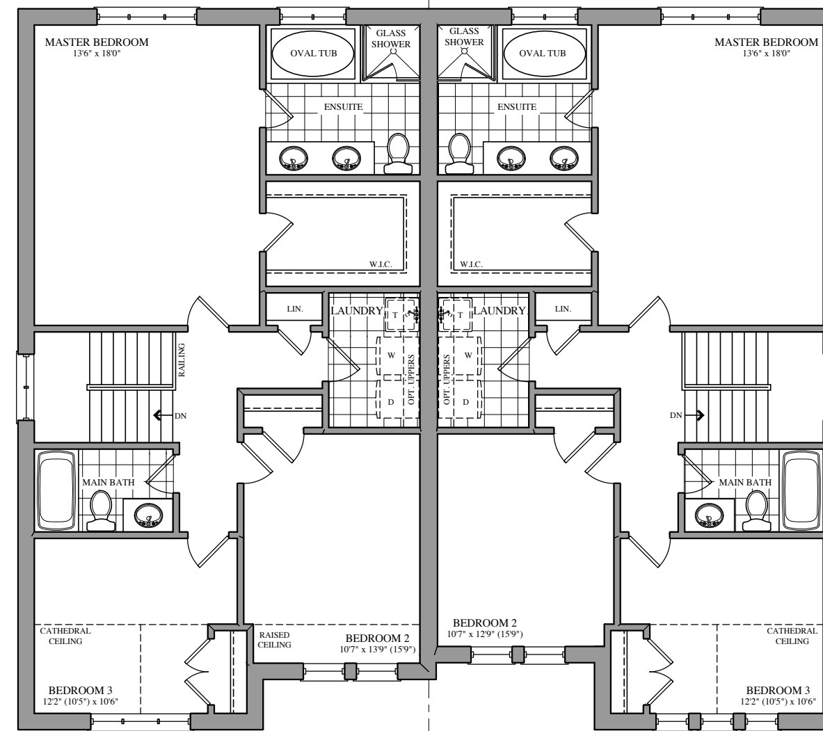
SECOND FLOOR PLAN ELEV. 'A'
