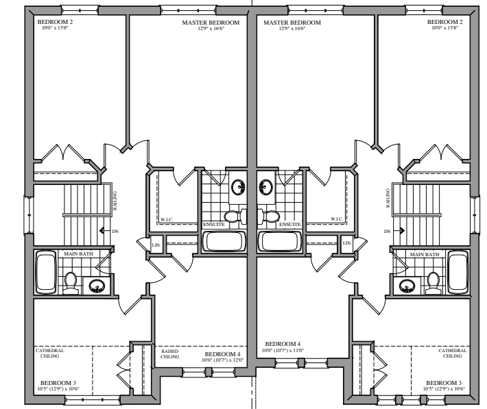
OPT. SECOND FLOOR PLAN ELEV. 'A'
