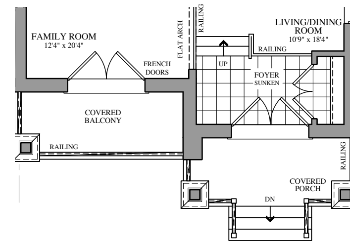
PART. GROUND FLOOR PLAN ELEV. 'D'
