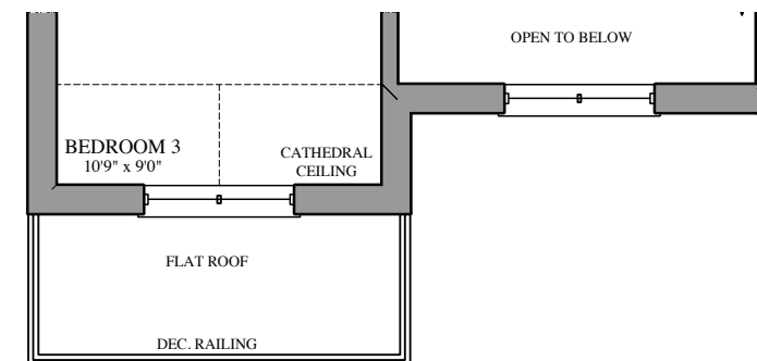
PART. SECOND FLOOR PLAN ELEV. 'C' & 'D'
