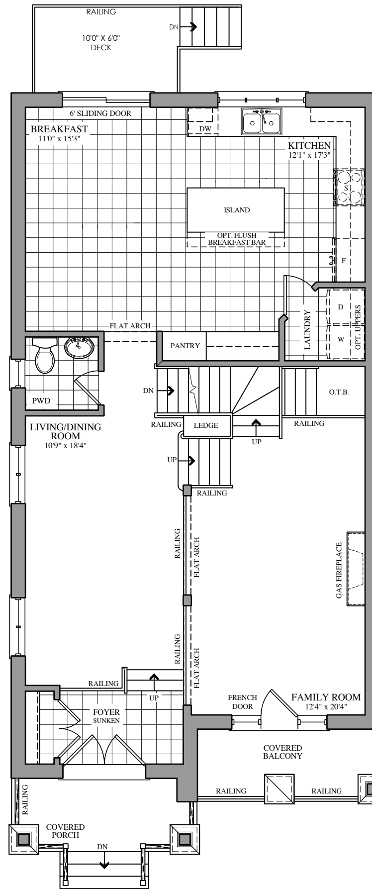
GROUND FLOOR PLAN ELEV. 'A' & 'B'
