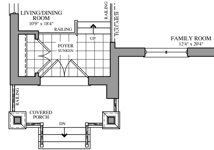
PART. GROUND FLOOR PLAN ELEV. 'C'
