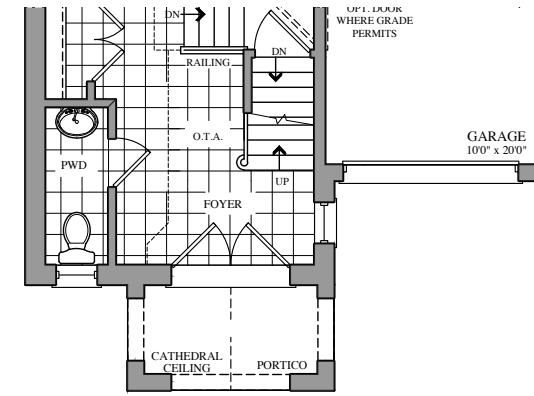
PART. GROUND FLOOR PLAN ELEV. 'C' & 'D'
