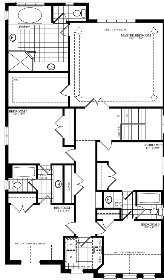
OPT. SECOND FLOOR W/ OPT. 5TH BEDROOM ELEVATION A
