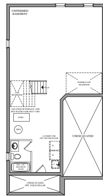
BASEMENT FLOOR PLAN ELEV. 'A' & 'B'
