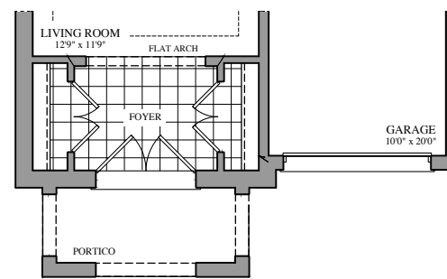
PART. GROUND FLOOR PLAN ELEV. 'C' & 'D'
