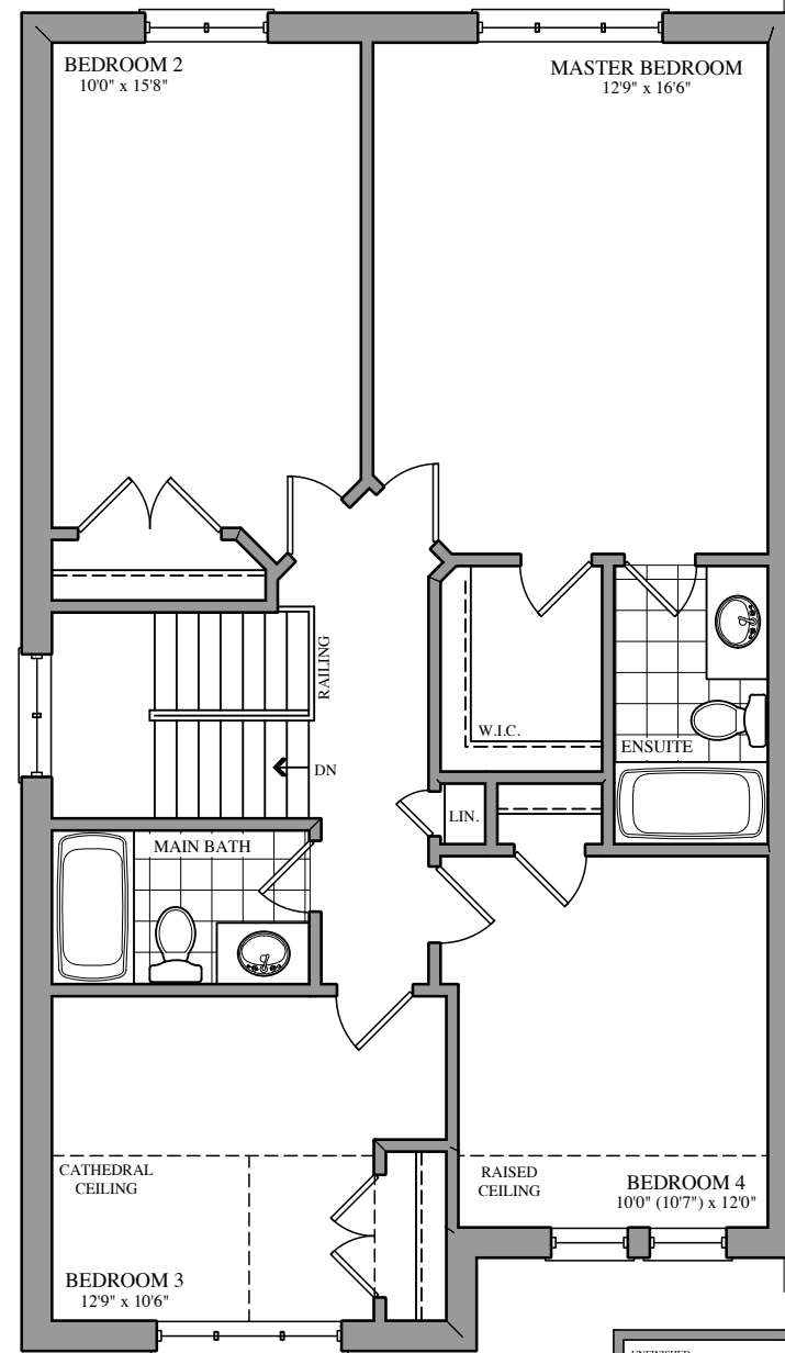
OPT. SECOND FLOOR PLAN ELEV. 'A'
