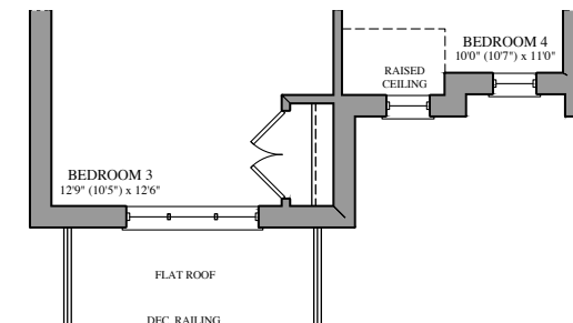
PART. OPT. SECOND FLOOR PLAN ELEV. 'C'
