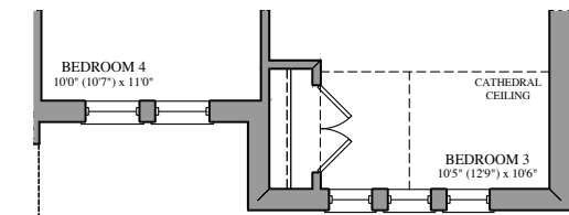
PART. OPT. SECOND FLOOR PLAN ELEV. 'B'
