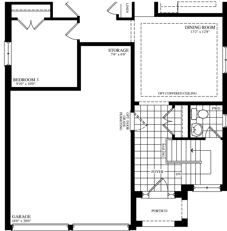
OPT. GROUND FLOOR ELEVATION A
