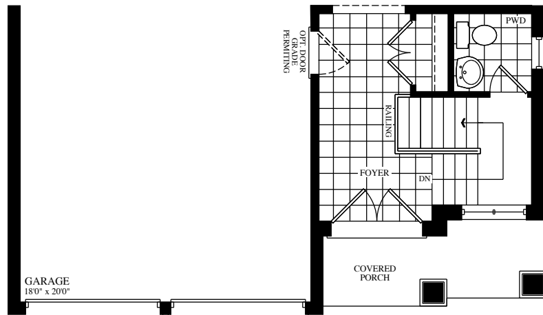
GROUND FLOOR ELEVATION B
