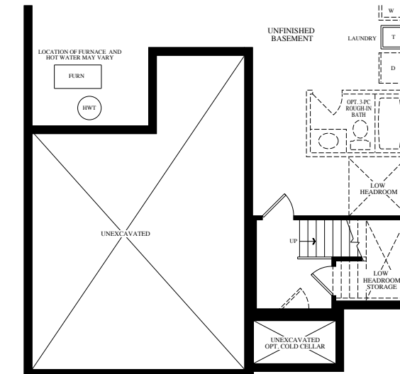
OPT. BASEMENT ELEVATION A
