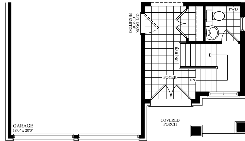
OPT. GROUND FLOOR ELEVATION B
