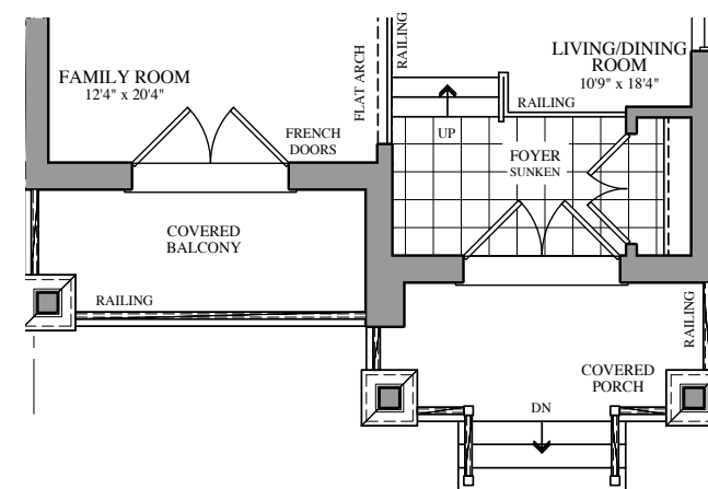
PART. GROUND FLOOR PLAN ELEV. 'D'
