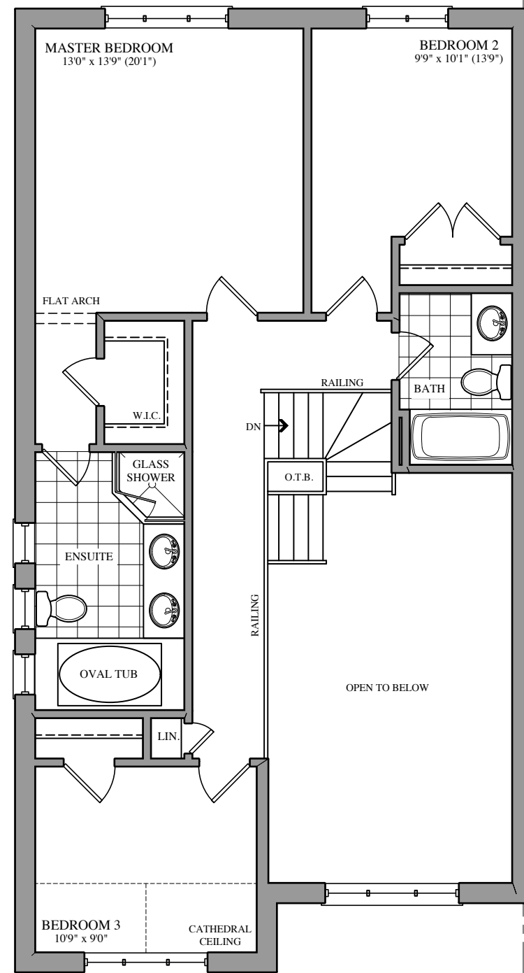
SECOND FLOOR PLAN ELEV. 'A' & 'B'
