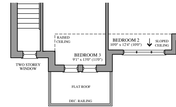
PART. SECOND FLOOR PLAN ELEV. 'C'
