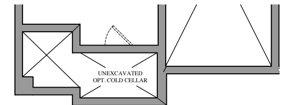
PART. BASEMENT FLOOR PLAN ELEV. 'C' & 'D'
