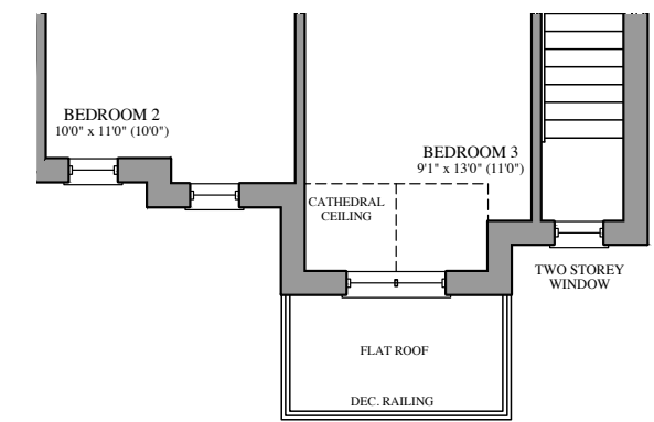
PART. SECOND FLOOR PLAN ELEV. 'D'
