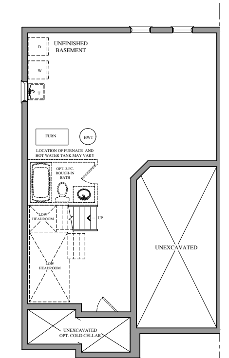
BASEMENT FLOOR PLAN ELEV. 'A'
