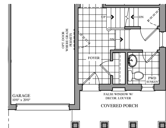
PART. GROUND FLOOR PLAN ELEV. 'B'
