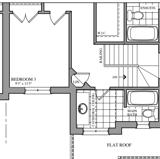
PART. SECOND FLOOR PLAN ELEV. 'D'
