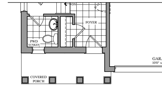
PART. GROUND FLOOR PLAN ELEV. 'C'
