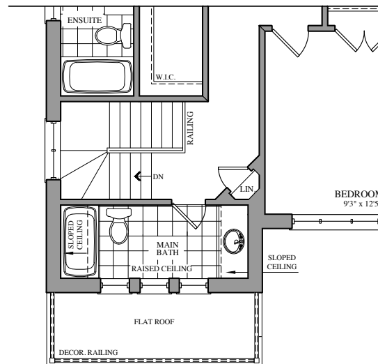
PART. SECOND FLOOR PLAN ELEV. 'C'
